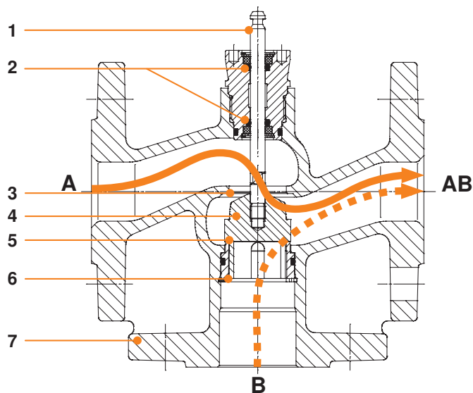
Section through an H7..N
