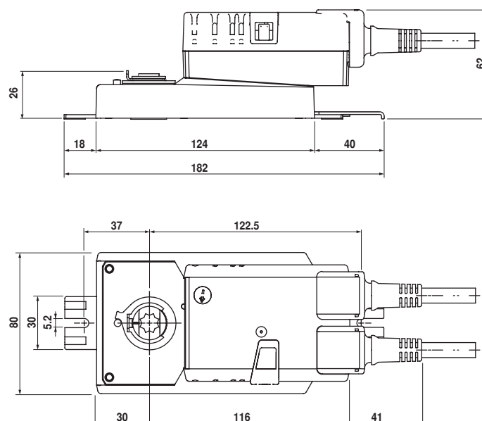
Dimensional drawings
